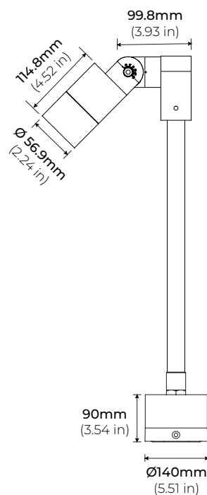
FL-811MP WITH LARGE ENCLOSURE BOX
