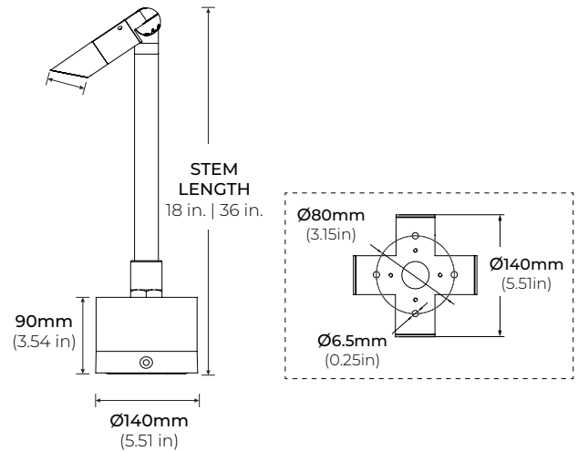
FL-801MP WITH LARGE ENCLOSURE BOX
