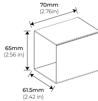
MOUNTING SLEEVE
